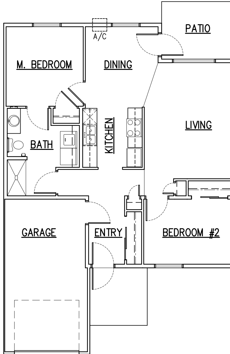
○ 2 BEDROOM UNIT 'A' 1/8" = 1'-0" 918 SF + 264 SF GARAGE
